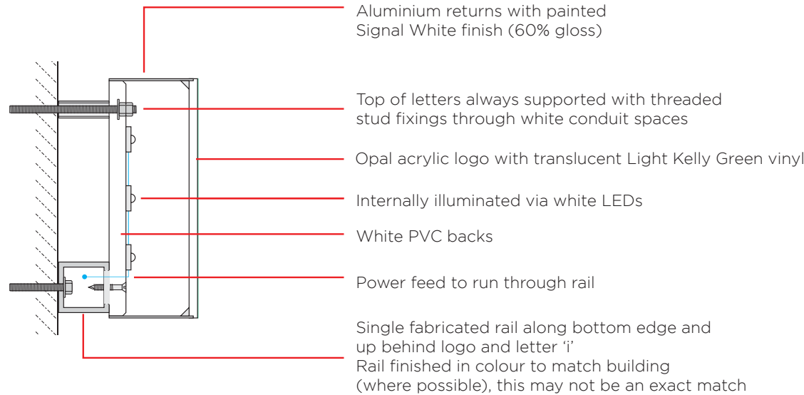
TYPICAL SECTION
